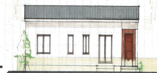
<South Elev>
